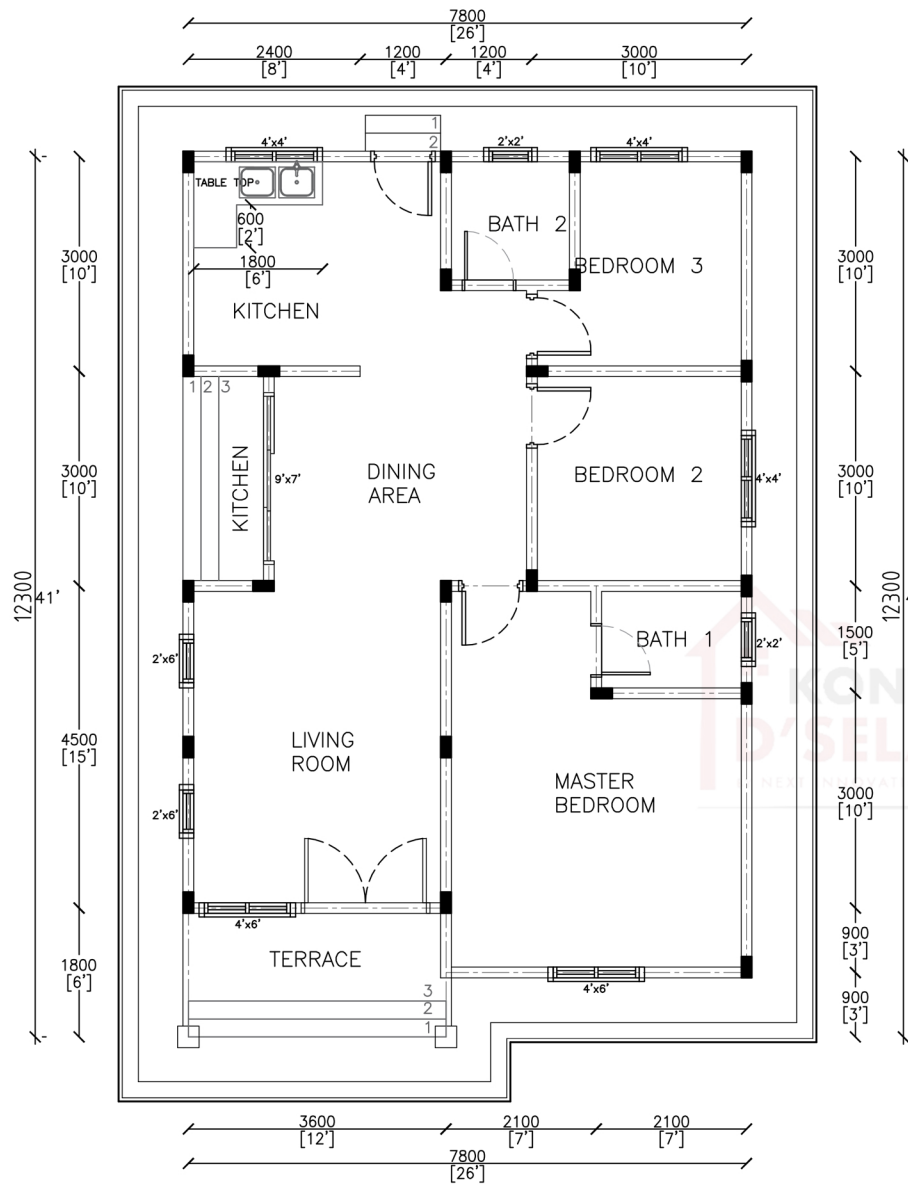
GROUND FLOOR PLAN SCALE : N.T.S
