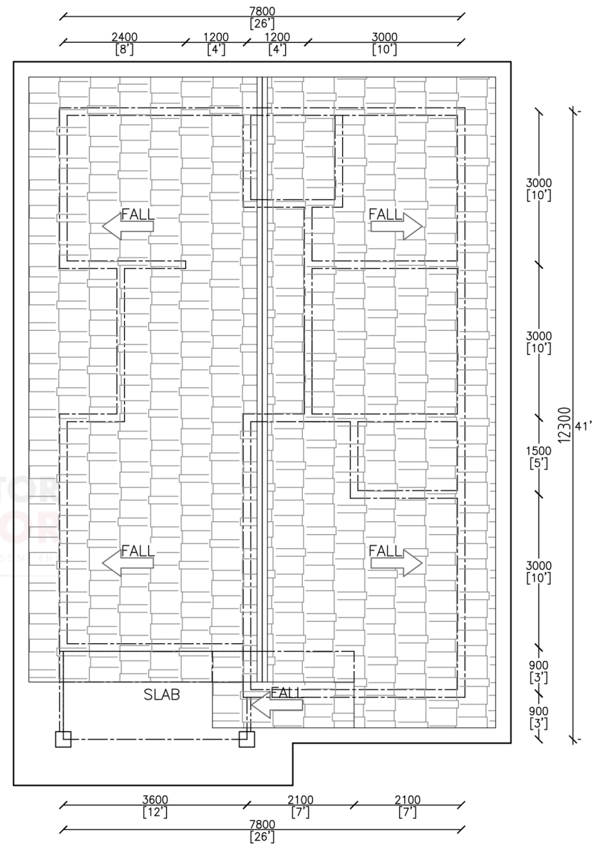
ROOF PLAN SCALE : N.T.S
