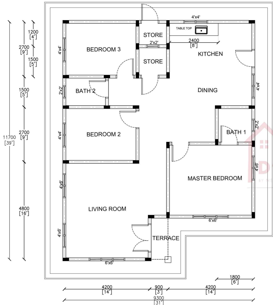
FLOOR PLAN
