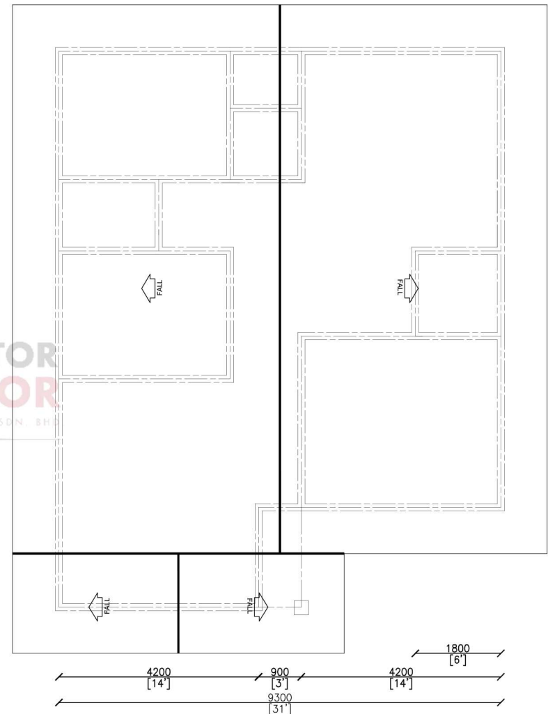
ROOF PLAN
