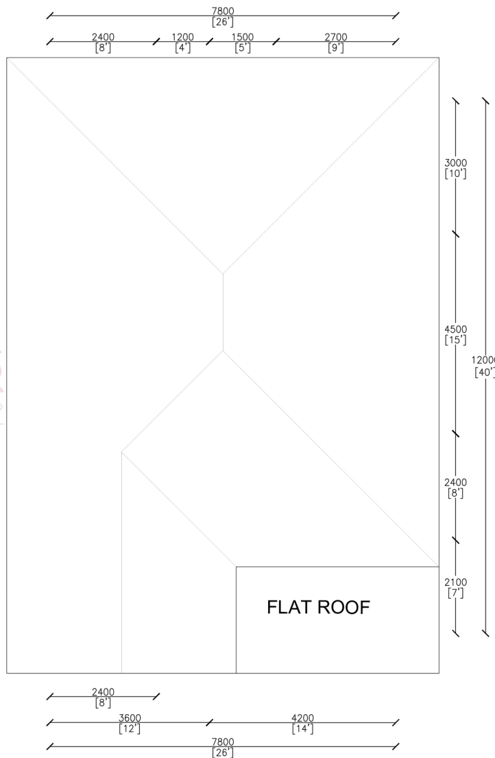
ROOF PLAN
