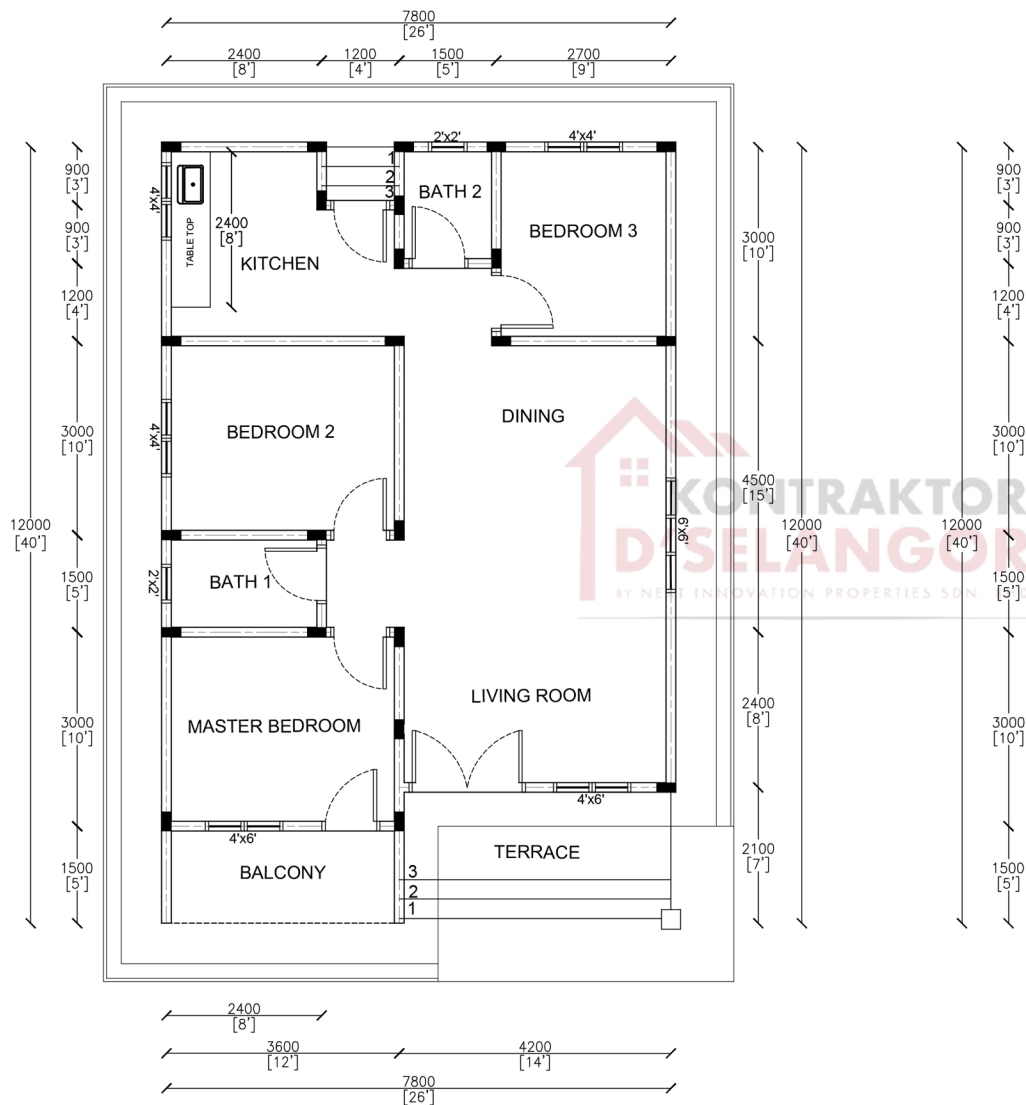
FLOOR PLAN
