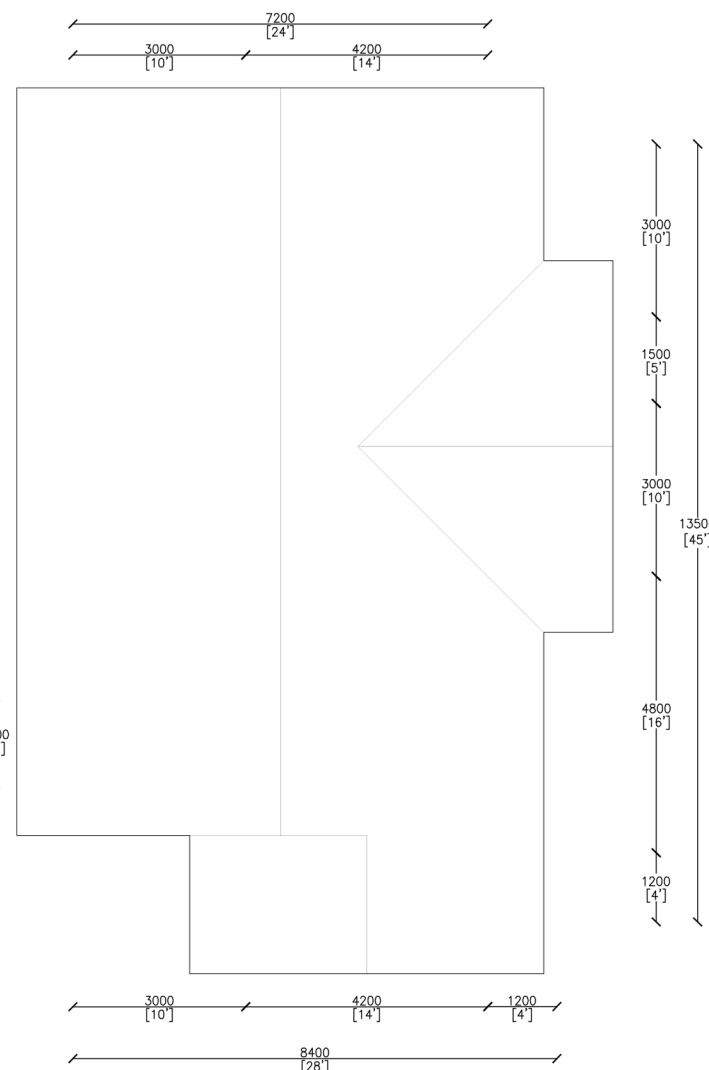
ROOF PLAN
