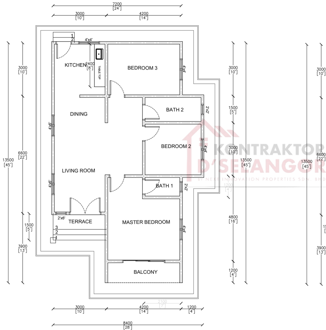
FLOOR PLAN
