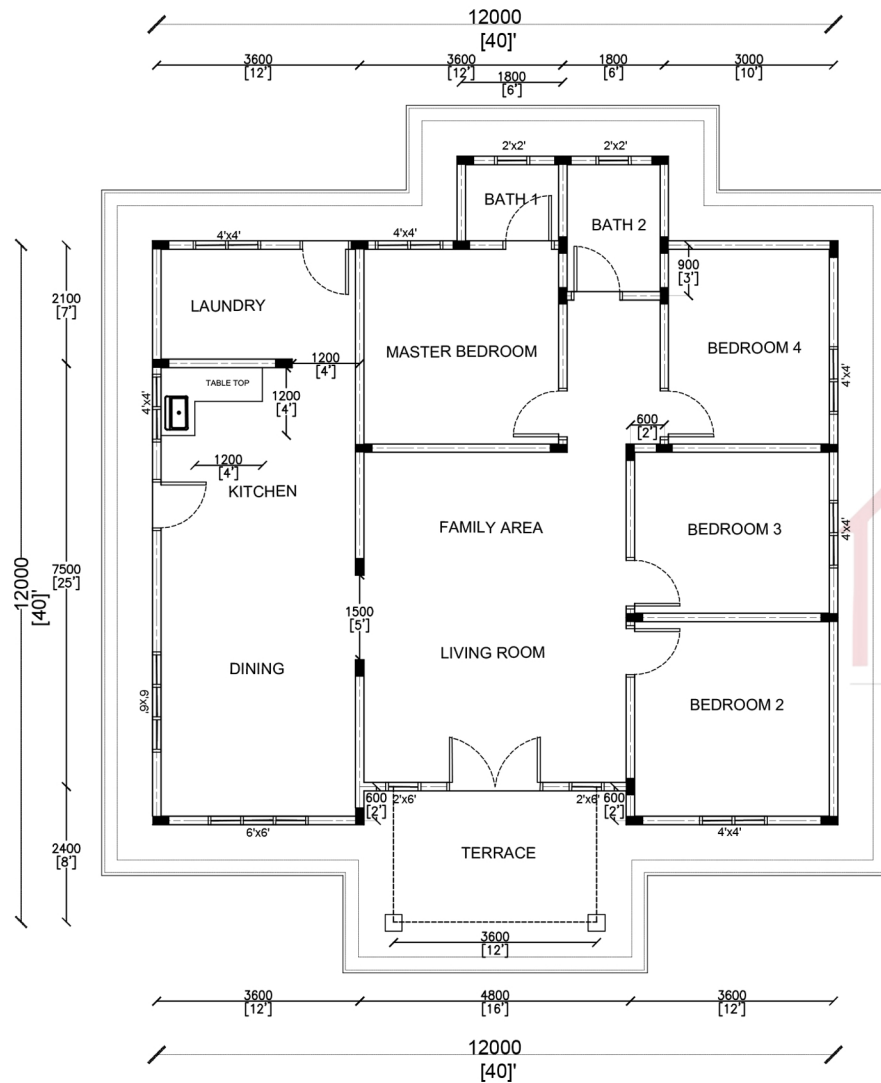
FLOOR PLAN
